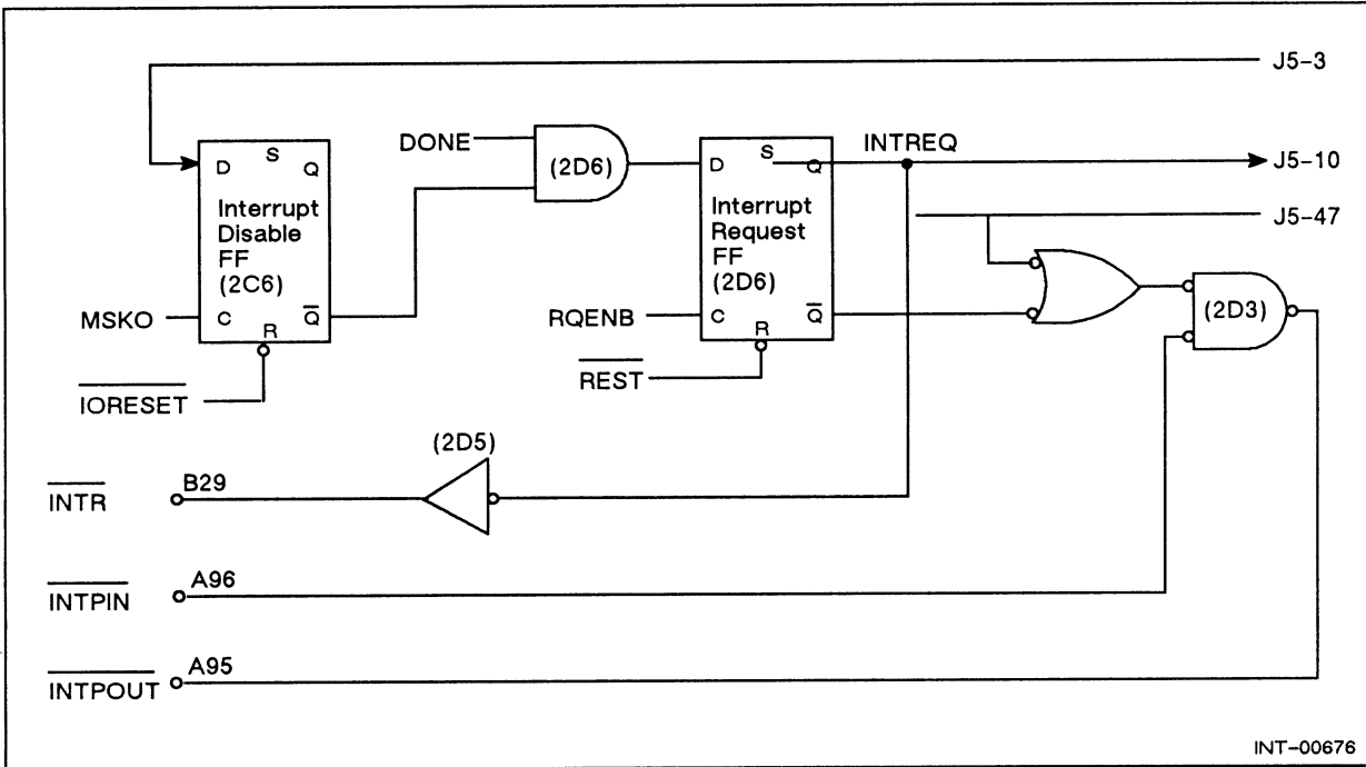
Figure 8-5 Model 4040A Interrupt Control Circuitry
