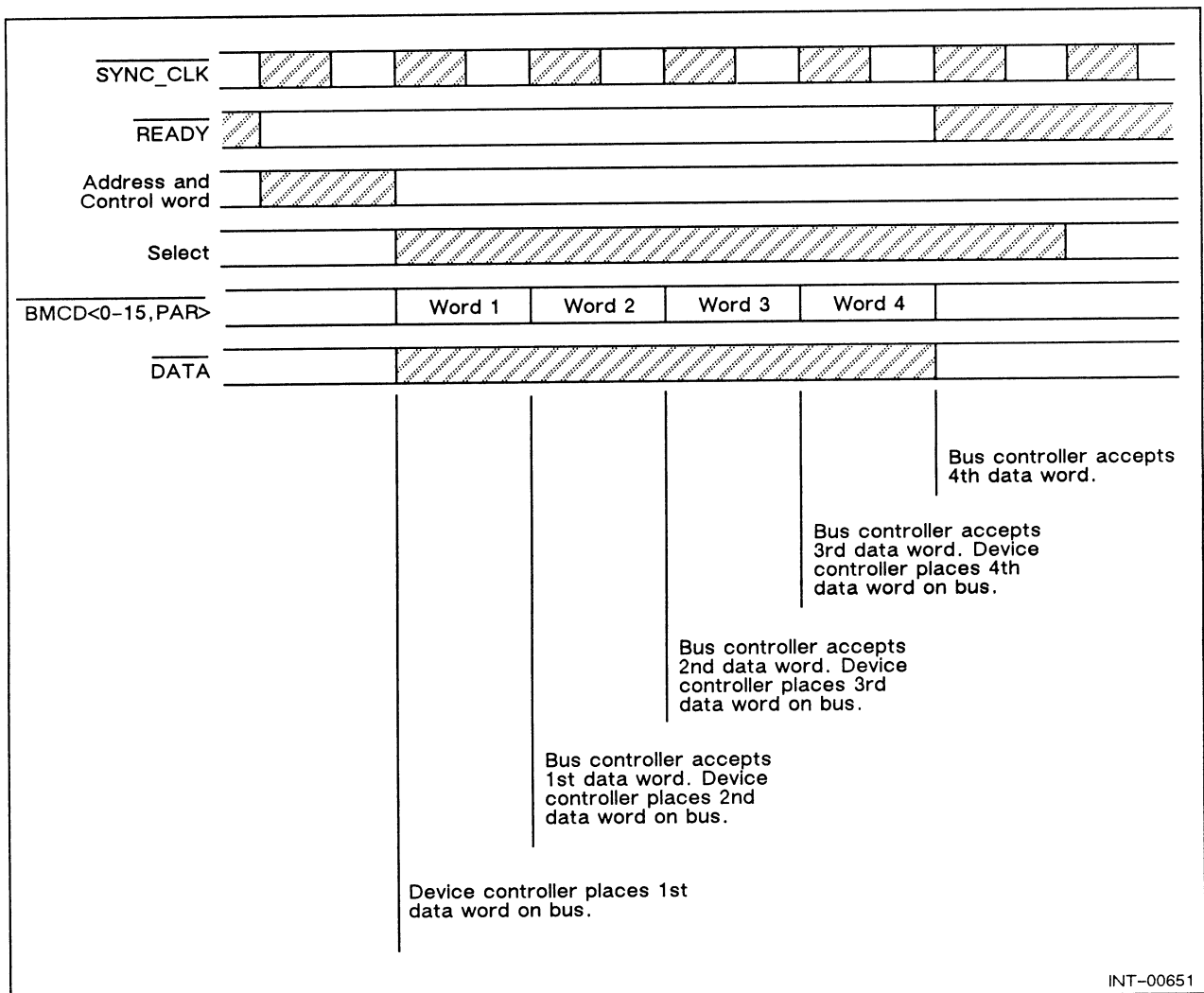
Figure 4–11 BMC Data Input Sequence
