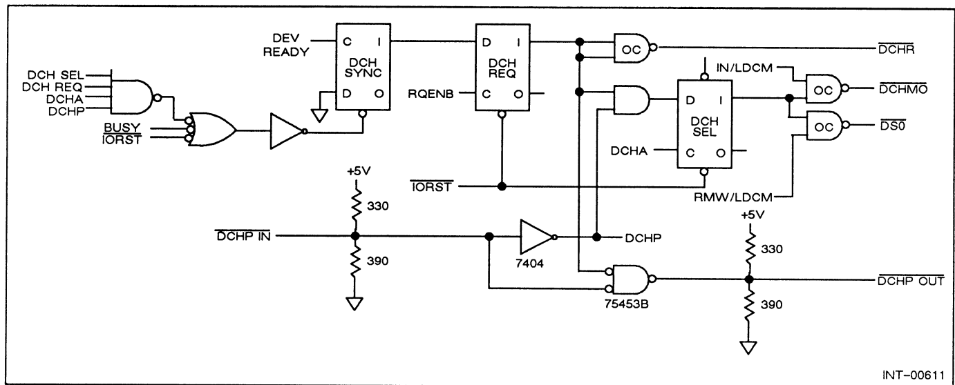
Figure 2-18 Typical Data Channel Control Circuit (Complete)
