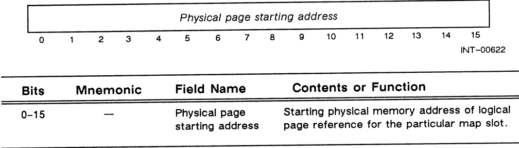
Figure 4-20 BMC Map Odd-Numbered Register Format (Low-Order Word)
