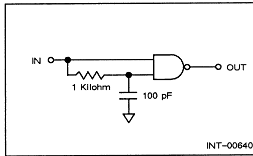
Figure 3-18 Bus Receiver
