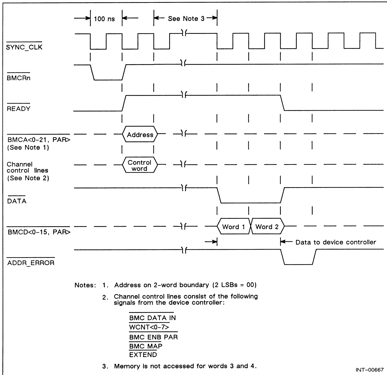
Figure 5-7 Data Output (1 Request, 4 Words, Protected Memory Error)
