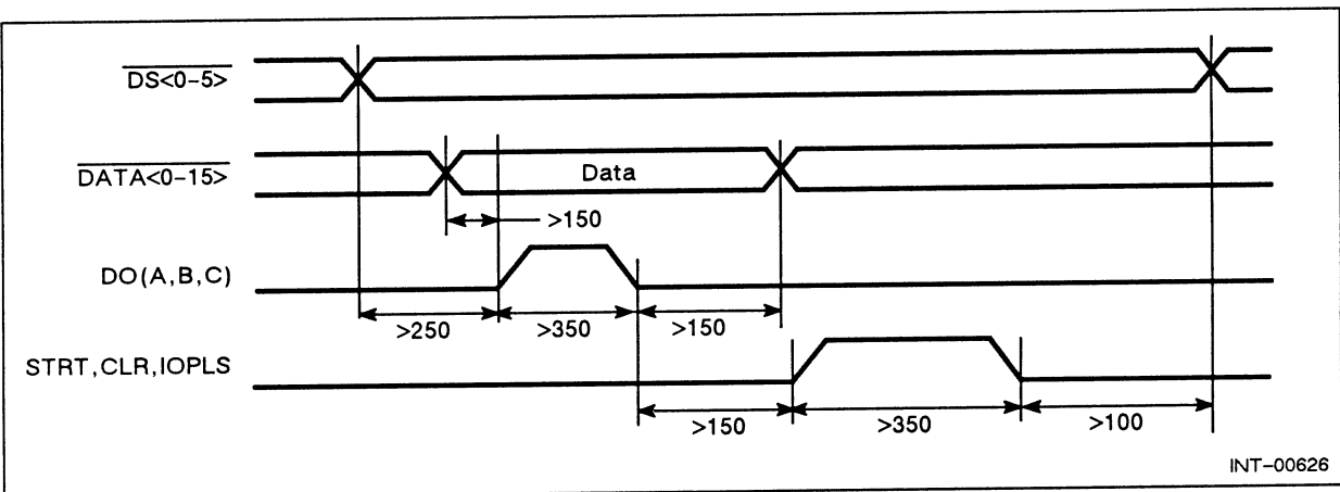
Figure 3-4 Programmed I/O Output with Start, Clear, or I/O Pulse
