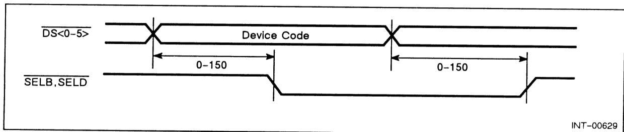
Figure 3-7 Skip Test
