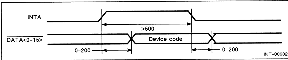
Figure 3-10 Interrupt Acknowledge
