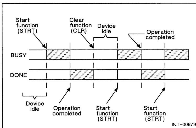
Figure 2-6 Busy/Done Sequencing
