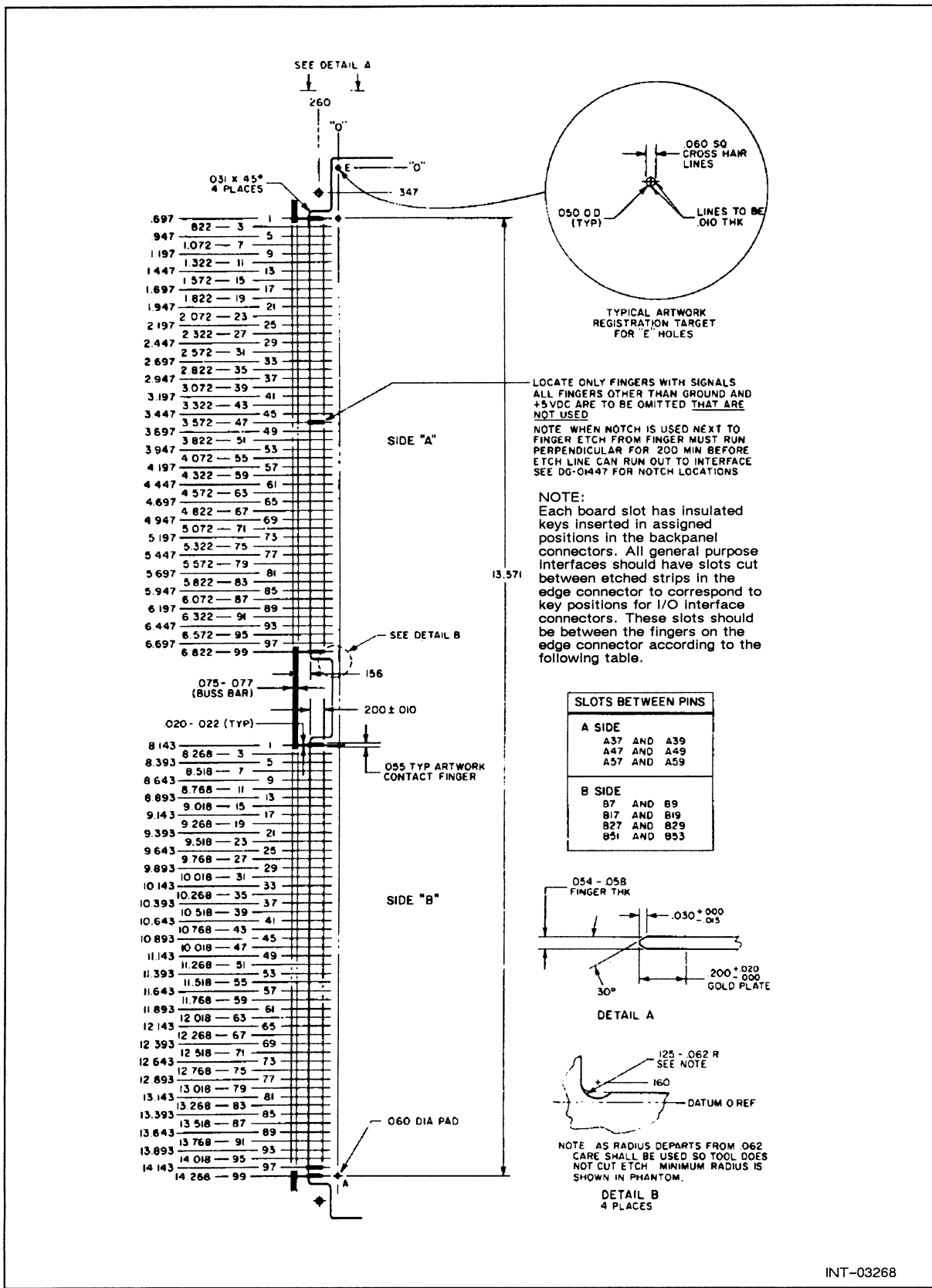
Figure 7-2 Connector Specifications
