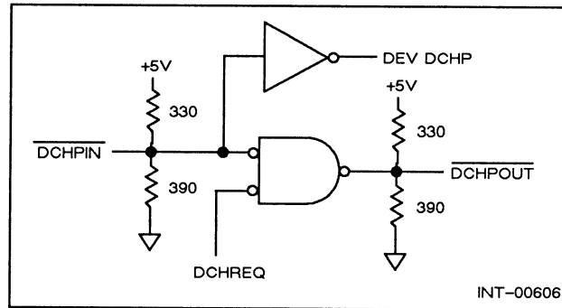
Figure 2-14 Typical Data Channel Priority Circuit
