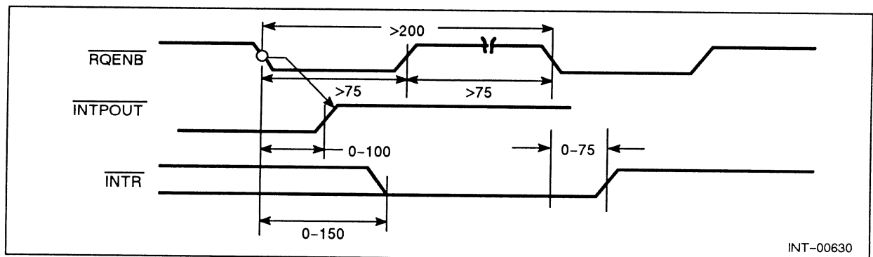
Figure 3-8 Program Interrupt
