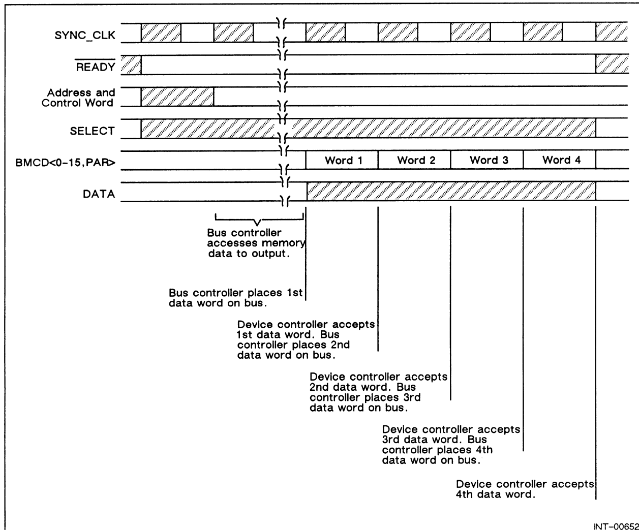
Figure 4-12 BMC Data Output Sequence
