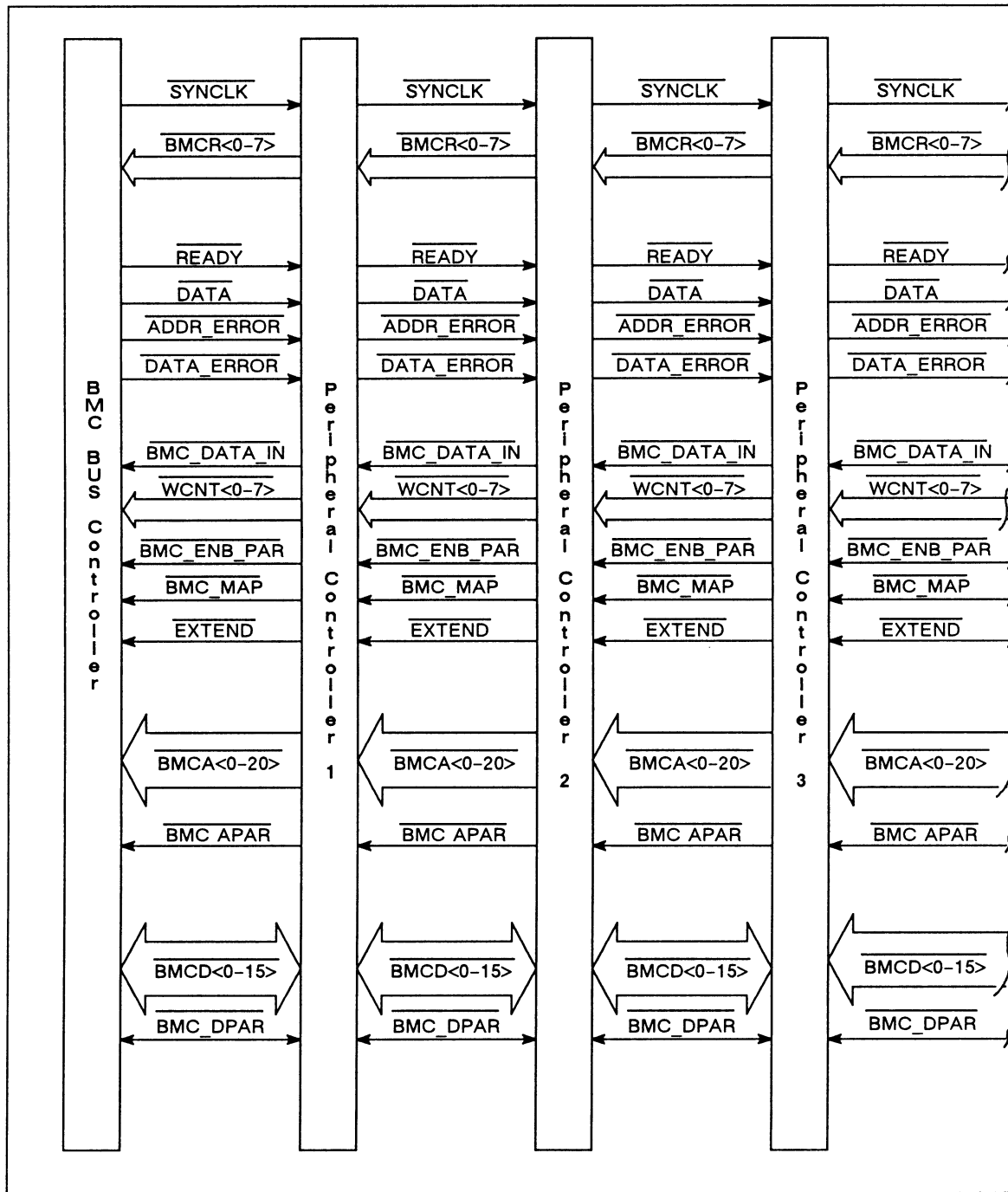
Figure 4-1 The BMC Bus
