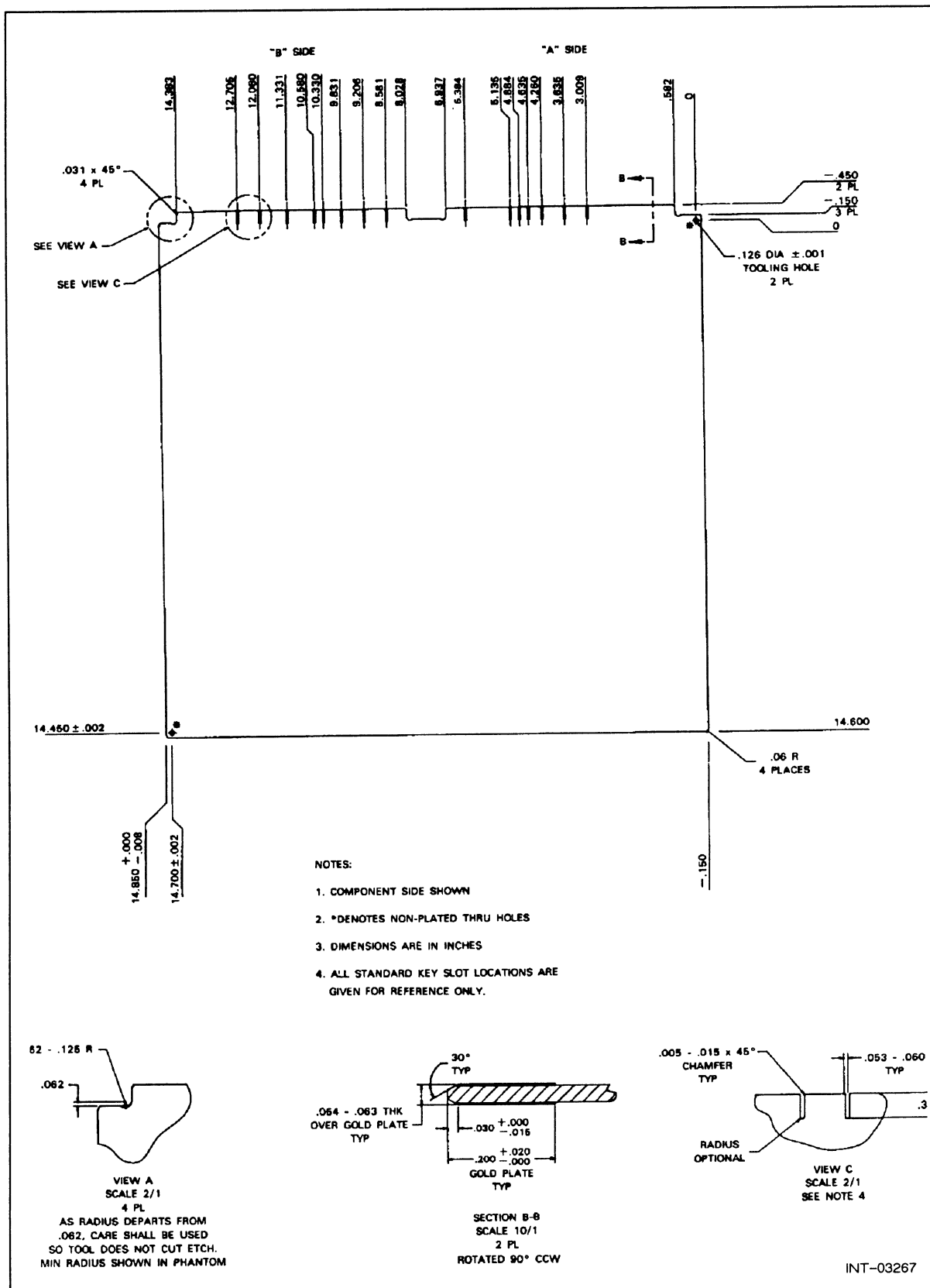
Figure 7-1 Mechanical Dimensions
