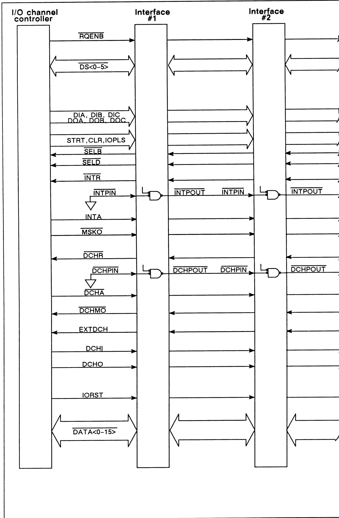
Figure 2-1 The I/O bus
