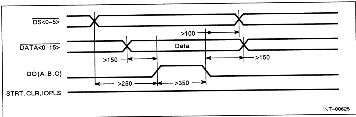
Figure 3-3 Programmed I/O Output Without Start, Clear, or I/O Pulse
