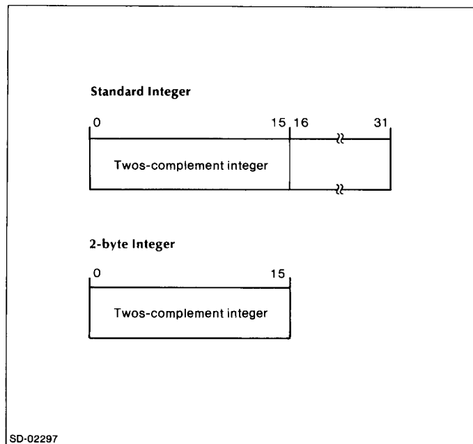
Figure 2-1. Internal Representation of an Integer
