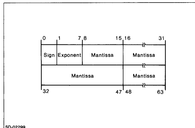
Figure 2-3. Internal Representation of a Double-Precision Number
