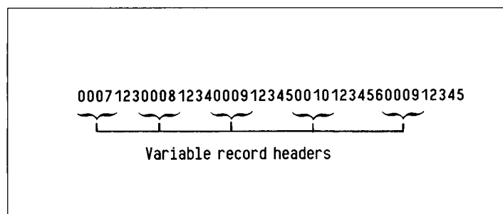
Figure E-1. Structure of Variable Records
