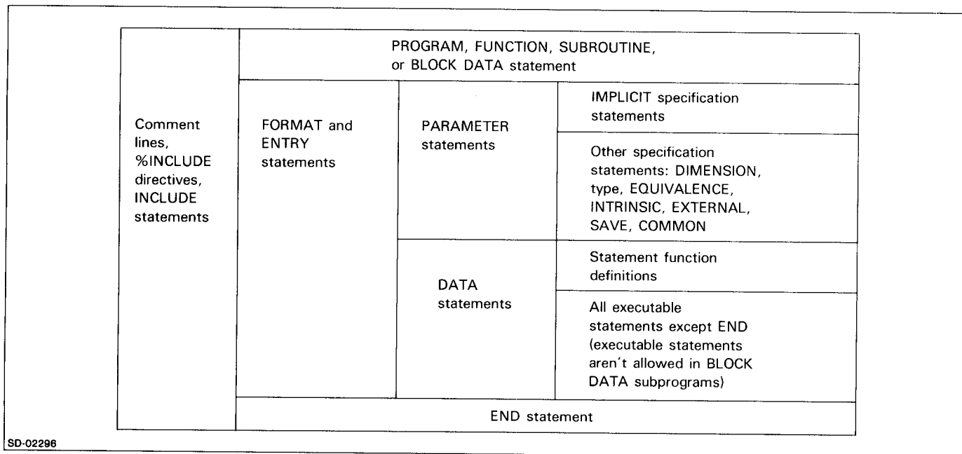
Figure 1-1. General Order of Statements in Program Unit
