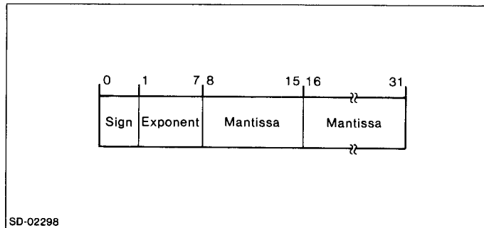
Figure 2-2. Internal Representation of a Real Number
